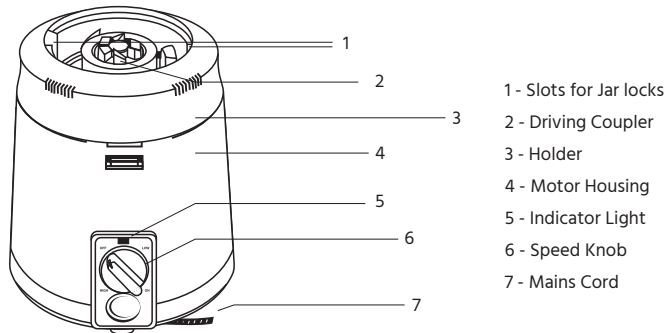
MOTOR UNIT
