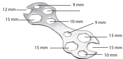
Multi purpose Spanner
