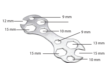
Multi purpose Spanner
